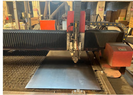
Laser cutting
